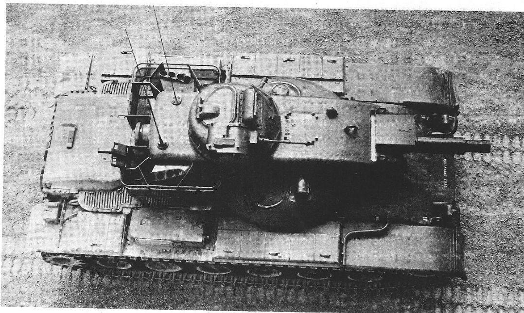
Figure 11-1. M60A2 tank. (Top view.)
