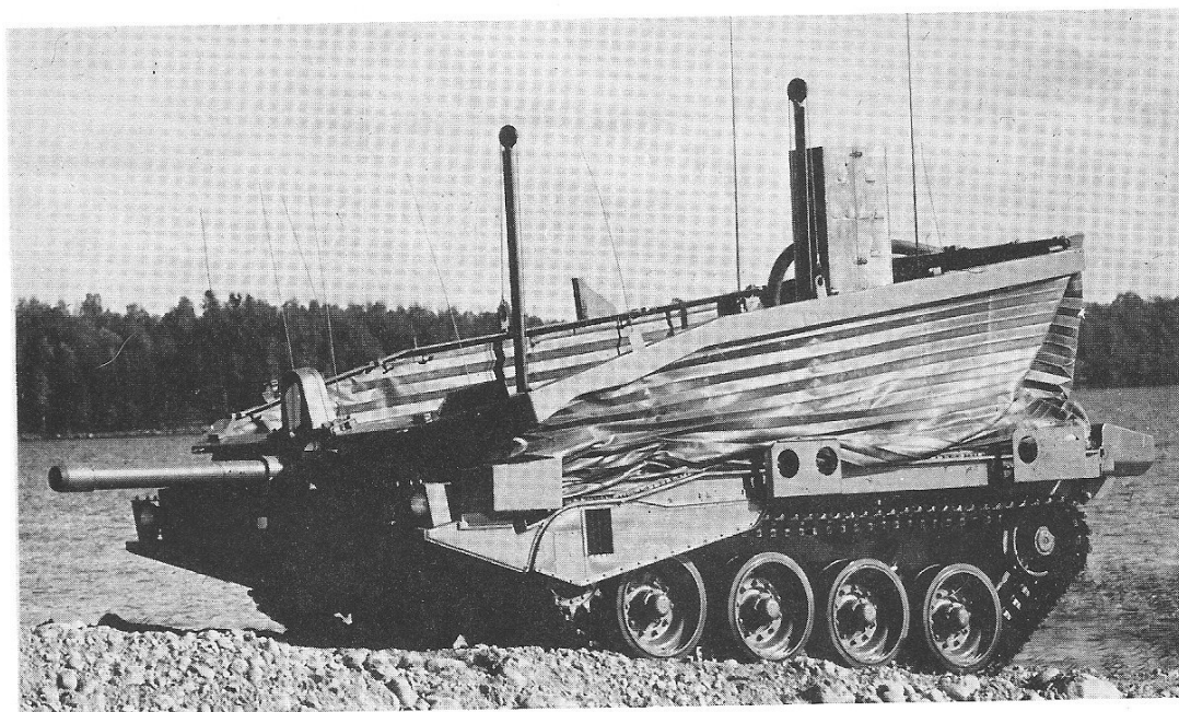
Figure 4-2. STRV-103 with erectable barriers.
